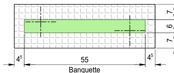
Implantation pied banquette 2.30m
