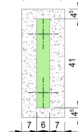
Implantation pied
